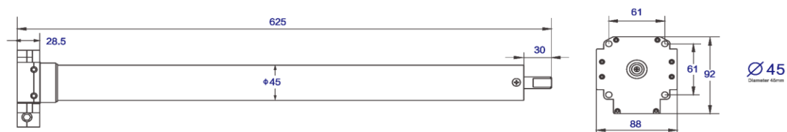
Motor Dimension
